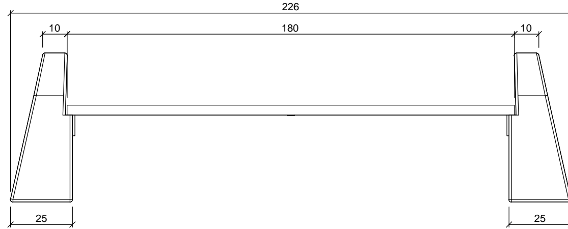
ALZADO / FRONT VIEW
